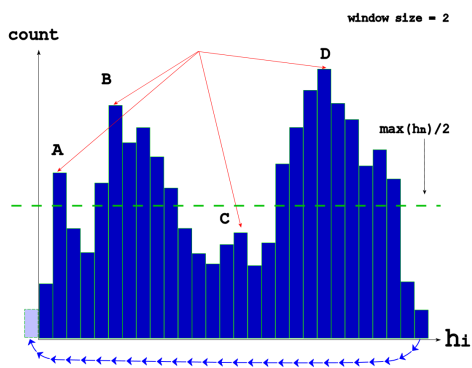
Figure 4: Vanishing point projection histogram
