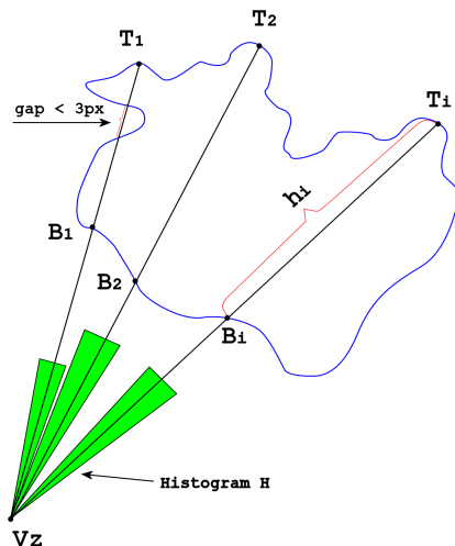
Figure 5: Vanishing point projection histogram
