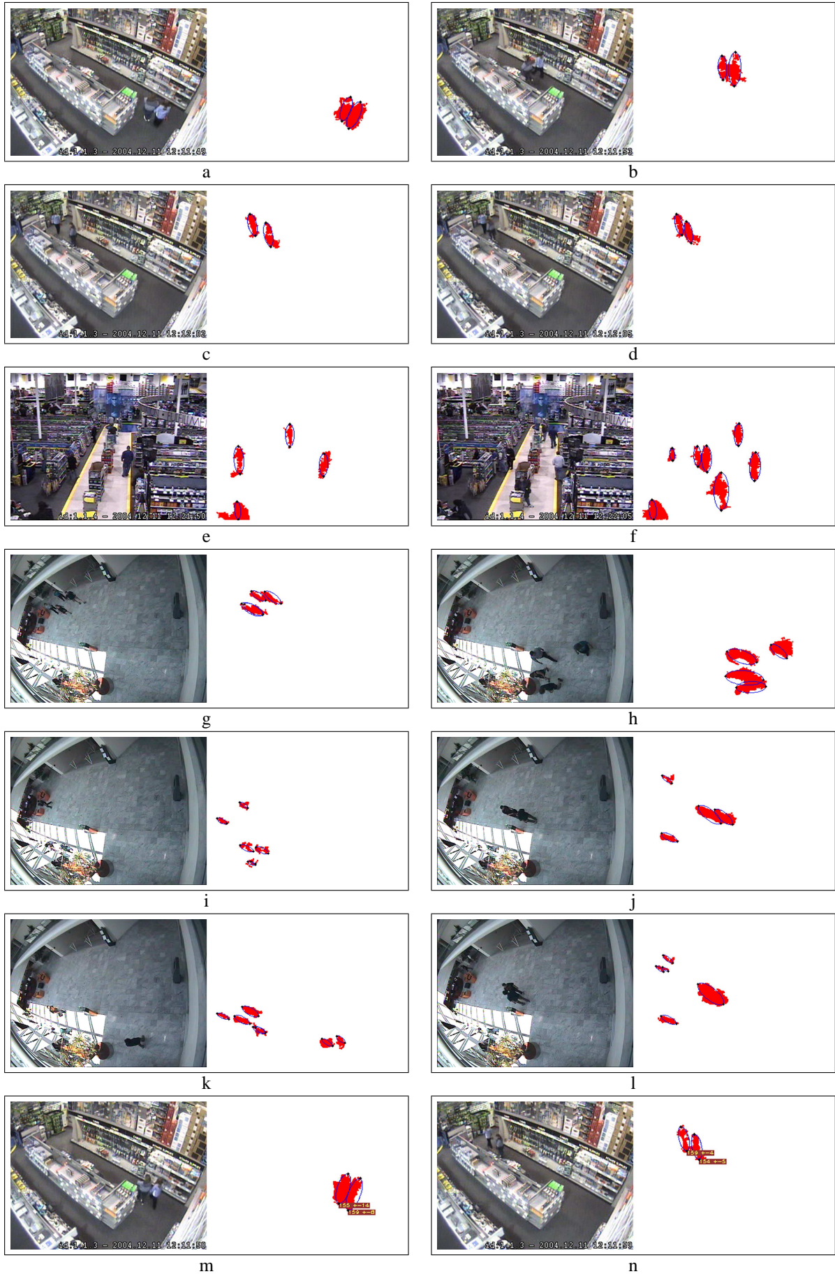
Figure 7: (a) - (l) Head candidates from test frames. Left image is the original frame. On the right image red represents foreground mask, small black dots indicate the locations of T_i and B_i ; blue ellipses are fitted with T_i B_i as the major axis; (m) and (n) Height detection: brown plates contain height mean and variance for each ellipse
